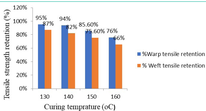
Figure 7: Effect of curing temperature on tensile strength.
