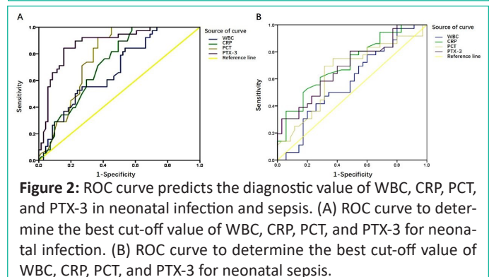
Figure 2: ROC curve predicts the diagnostic value of WBC, CRP, PCT, and PTX-3 in neonatal infection and sepsis. (A) ROC curve to determine the best cut-off value of WBC, CRP, PCT, and PTX-3 for neonatal infection. (B) ROC curve to determine the best cut-off value of WBC, CRP, PCT, and PTX-3 for neonatal sepsis.
