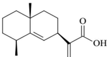
Figure 1: Chemical structure of pterodontic acid .
