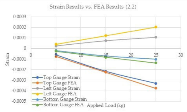
Figure 24: Validated FEA of each gauge.
