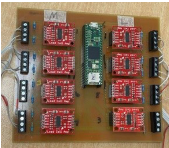
Figure 19: Printed circuit board.
