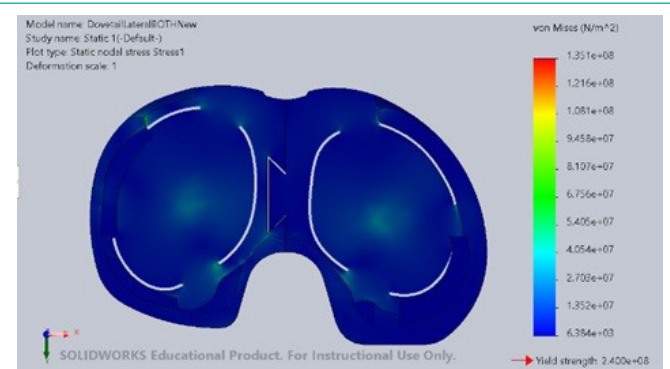
Figure 14: Stress distributions (stress raises at tabs).
