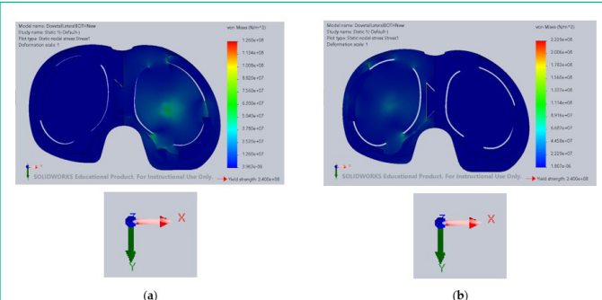
Figure 15: Stress from 700 N point load (a) Load applied to medial compartment (b) Load applied to lateral component.
