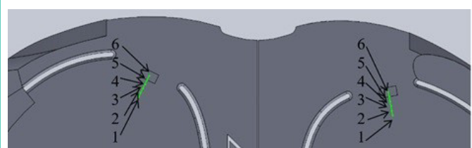
Figure 12: Locations of stress raises towards strain gauges.
