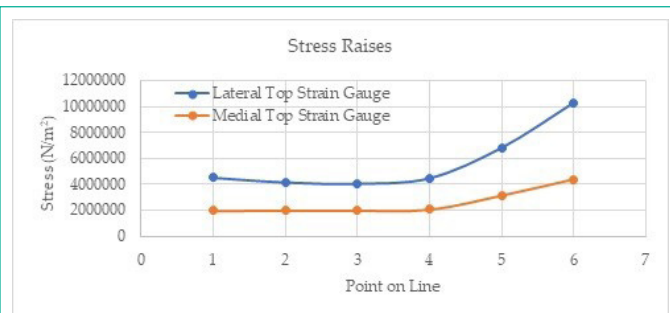
Figure 13: Stress raises results.
