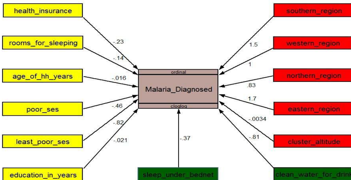
Figure III: The G-SEM pathway diagram shows direct coefficients from ordinal regression analysis of the effects of selected random predictor variables on malaria infection outcome variables resulting in children and adults in Rwanda in 2010. Key for variables names: individuals covered by health insurance (health_insurance), number of rooms for sleeping in each house (rooms_for_sleeping), age of household members in years (age_of_hh_years), poor SES versus most poor SES (poor_ses), least poor SES versus most poor SES (least_poor_ses), education gain of each household member in years (education_in_years), number of household members sleep under a treated mosquito bed net (sleep_under_bednet), household members have a clean water excess for drinking (had_water_excess), cluster altitude in meters (cluster altitude), the eastern region of Rwanda (eastern_region), the northern region of Rwanda (northern_region), the western region of Rwanda (western_region), the southern region of Rwanda (southern_region). Other: the arrows pointing from the exogenous (explanatory variables) to endogenous (dependent variable).
