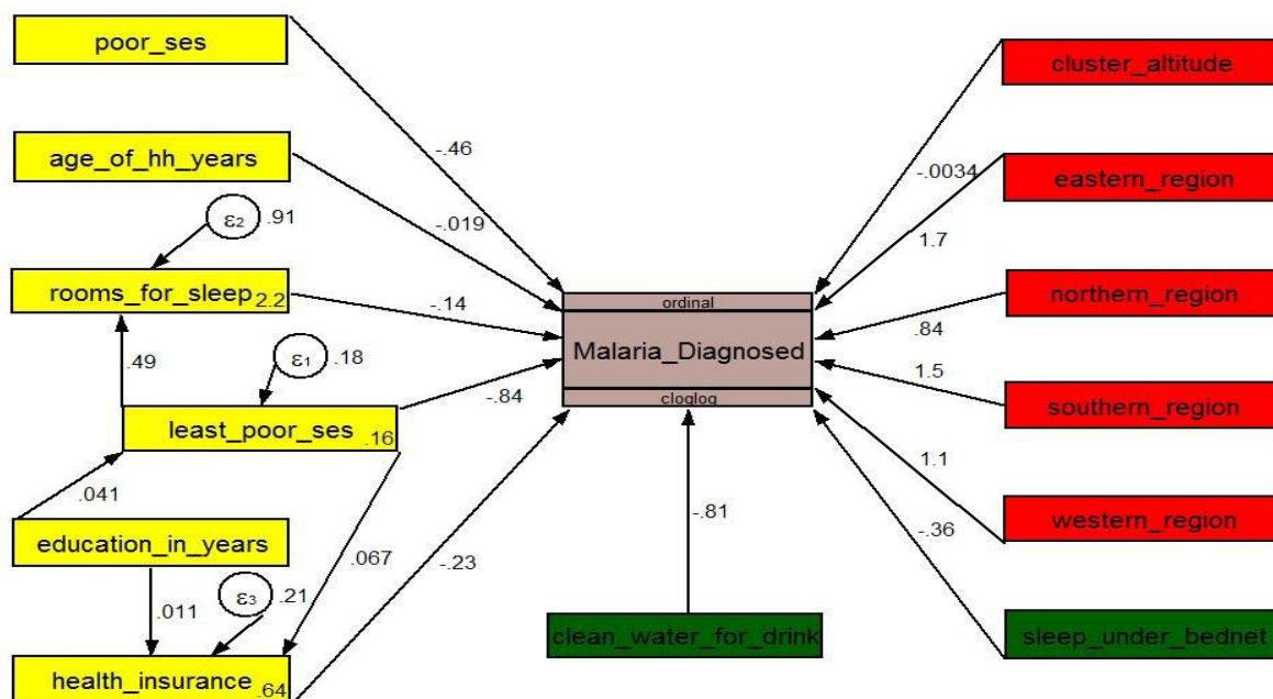
Figure IV: Diagram shows direct and indirect pathways and coefficients from G-SEM based ordinal regression analysis of the effects of selected random predictor variables on malaria infection outcome variable result in children and adults in Rwanda in 2010. Key for variables names: individuals covered by health insurance (health_insurance), number of rooms for sleeping in each house (rooms_for_sleeping), age of household members in years (age_of_hh_years), poor SES versus most poor SES (poor_ses), least poor SES versus most poor SES (least_poor_ses), education gain of each household member in years (education_in_years), number of household members sleep under a treated mosquito bed net (sleep_under_bednet), household members have a clean water excess for drinking (had_water_excess), cluster altitude in meters (cluster altitude), the eastern region of Rwanda (eastern_region), the northern region of Rwanda (northern_region), the western region of Rwanda (western_region), the southern region of Rwanda (southern_region). Other: the arrows pointing from the exogenous (explanatory variables) to endogenous (dependent variable) and the error terms placed on all three endogenous variables.
