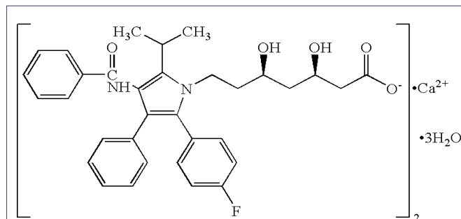
Figure 1: Atorvastatin Calcium.
