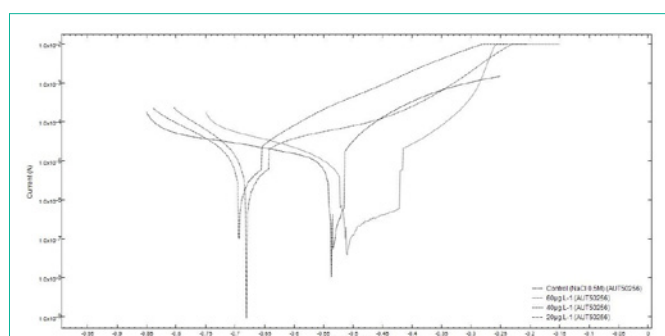
Figure 4: Polarization curves for AISI 1020 carbon steel in the salting medium (NaCl 0.5M) in the presence of different concentrations of L. gracilis Schauer essential oil using as control NaCl (0.5M).
