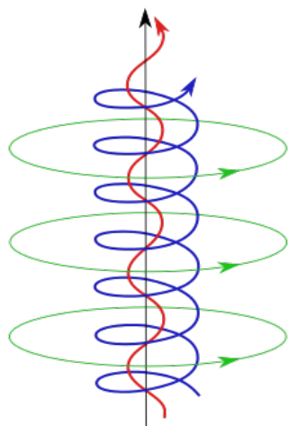
Figure 2: The complex self-constricting magnetic field lines and current paths in a field-aligned Birkeland current that can develop in a plasma
