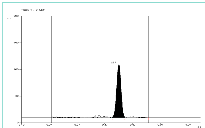
Figure 11: Densitogram of API of Leflunomide (150 ng/band) and its degradation products in the thermal degradation study using mobile phase n-Hexane: Ethyl Acetate (7:3 v/v).
