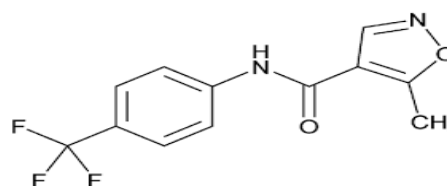
Figure 1: Chemical structure of Leflunomide.
