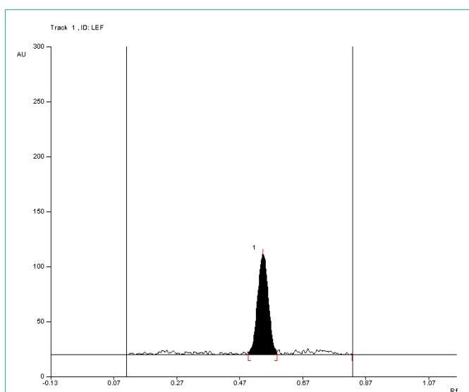
Figure 13: Densitogram of API of Leflunomide (150 ng/band) and its degradation products in the photolytic degradation study using mobile phase n-Hexane: Ethyl Acetate (7:3 v/v).
