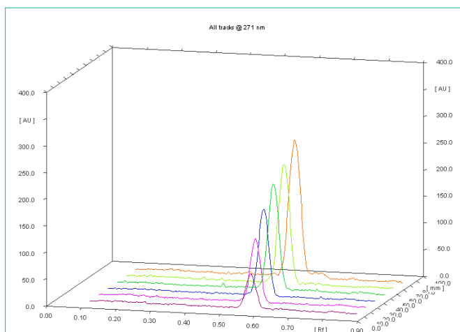
Figure 15: Three dimensional overlay of HPTLC densitogram of calibration bands of Leflunomide.
