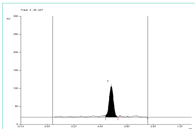
Figure 14: Densitogram of sample of Leflunomide (150 ng/band) and its degradation products in the photolytic degradation study using mobile phase n-Hexane: Ethyl Acetate (7:3 v/v).
